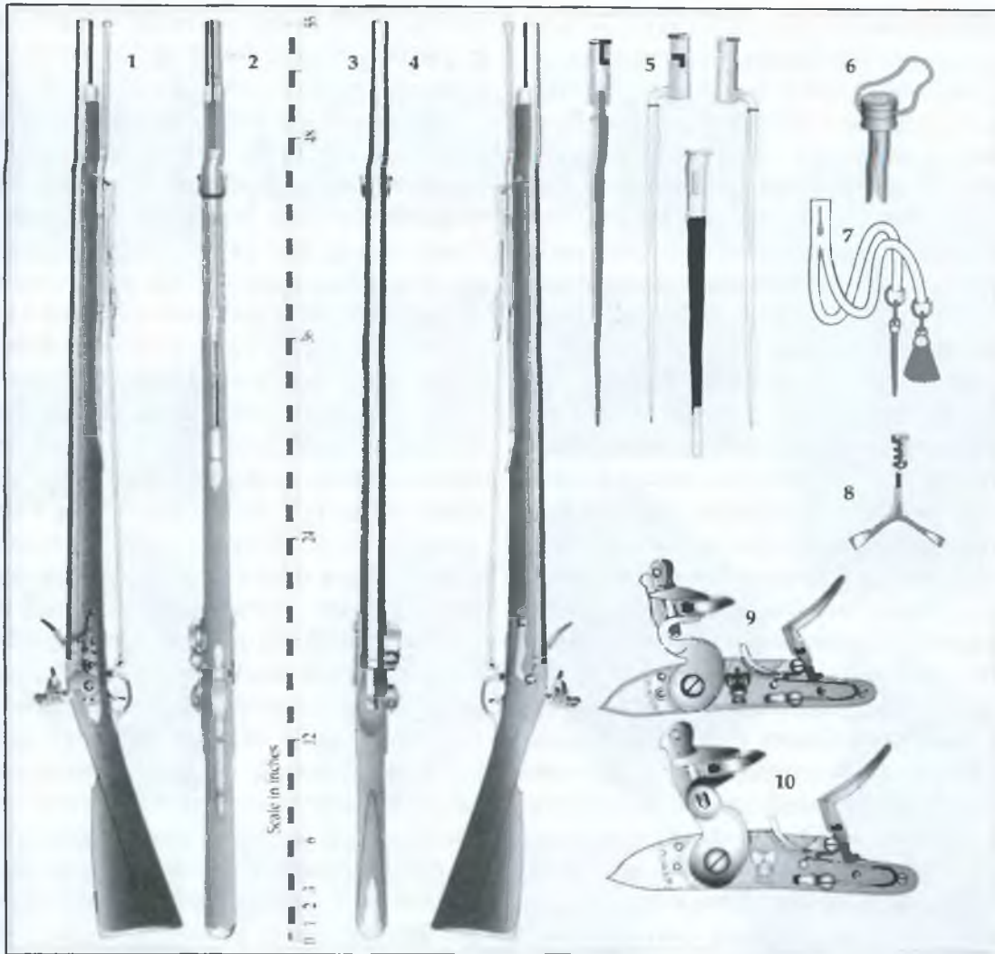
India Pattern Musket. A right side view showing the earlier swan necked lock (1), an under view showing the three pipes for the ramrod (2) and an upper view (3). A left side view showing the simple side plate (4). Views of the regulation bayonet and scabbard (5). A muzzle bung used to exclude the ingress of dirt and rain into the bore (6) and the picker and brush usually worn attached to a button behind the breast plate of the jacket (7). The combination tool for the musket (8) and views of the early pattern swan necked lock of circa 1797, (9) and the later pattern swan necked lock of circa 1809 (10).
